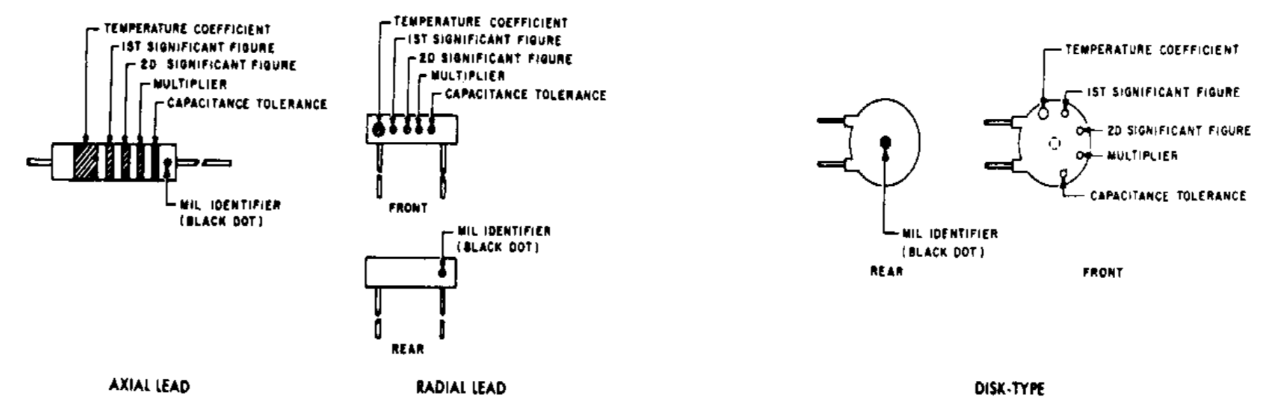
Figure 121. Color code marking for military standard capacitors.
