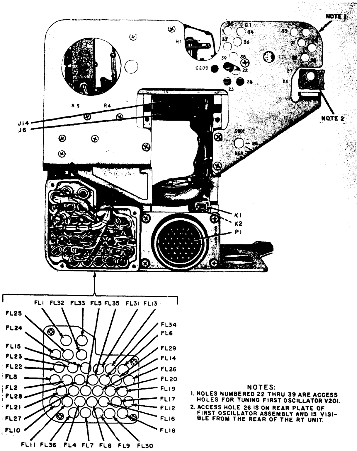
Figure 48. Main frame, rear view.
