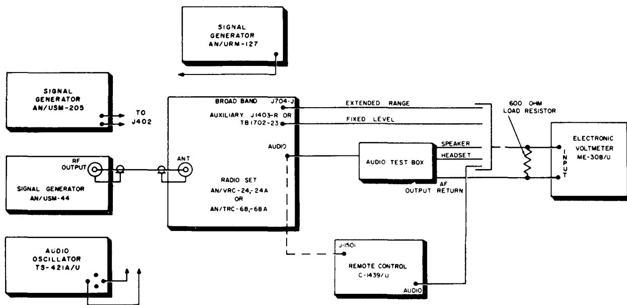
Figure 118. Receiver audio output and audio level adjustment test.
